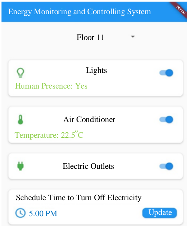
Fig. 2 Mobile application interface of the system
