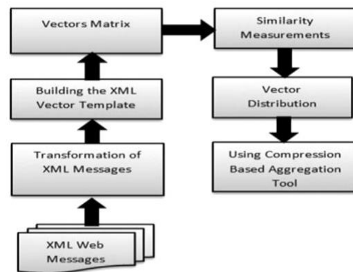
Figure 2. Architect model for SOAP massaging vector
