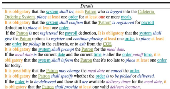
Fig. 2. SBVR rule representation of software requirements
